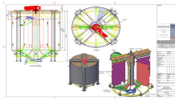
Design of high water-temperature flotation chamber
